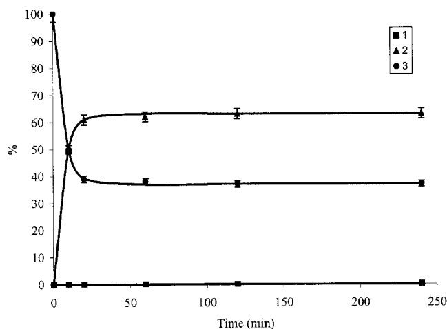
Figure 3. Diacetate proportions from 3 in THF
