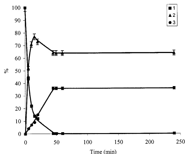
Figure 1. Diacetate proportions from 1 in THF
