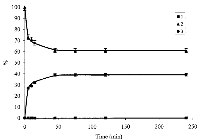
Figure 2. Diacetate proportions from 2 in THF
