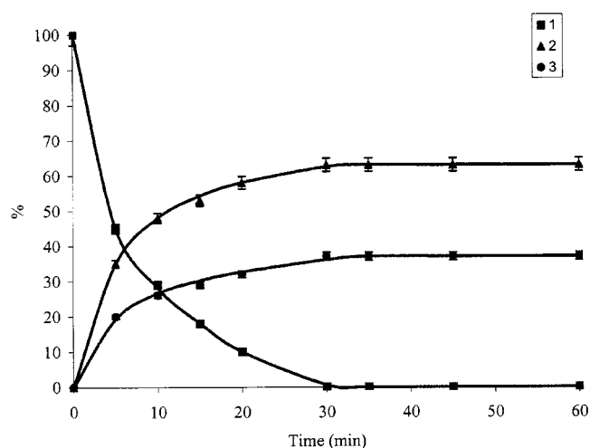
Figure 4. Diacetate proportions from 1 in DMF
